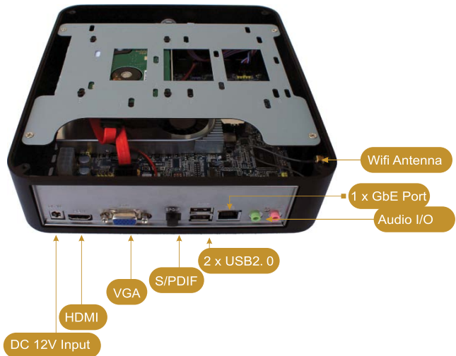
Rear I/O:
